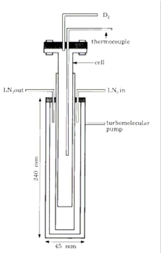
Fig. 2 - The titanium cell and the cryostat
