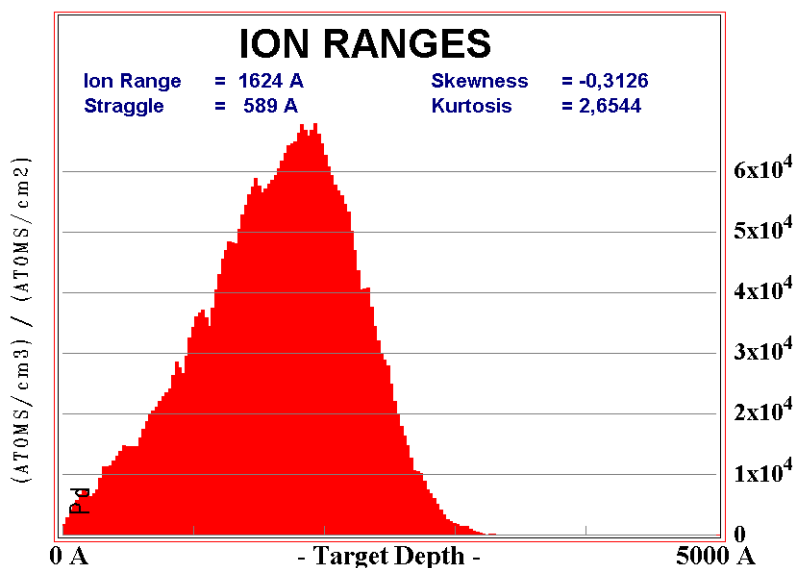
Fig. 1 - Boron ions distributions vs. target depth
