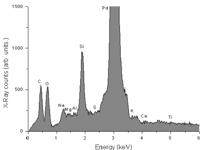
Fig. 5 - EDX spectrum of a sample with 76 days of treatment (by D 2 gas only). We can observe the presence of the following elements:
